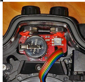
Optoelectronic TTL-Converter for SONY A1 and A7-A9 for NAUTICAM underwater housings
