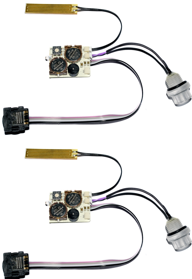
16023 TTL-Converter for Sony A7-A9 line for IKELITE housings
